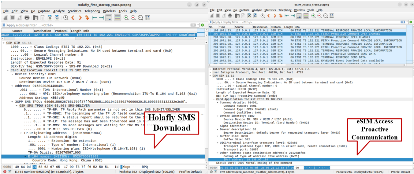
Figure 10: Wireshark showing the captured proactive communication for eSIM Access and Holafly.
