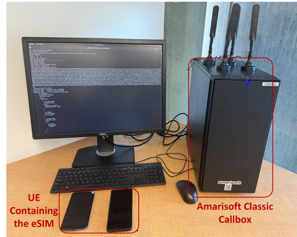
Figure 8: An eSIM was connected to our private network to capture logs and conduct experiments.
